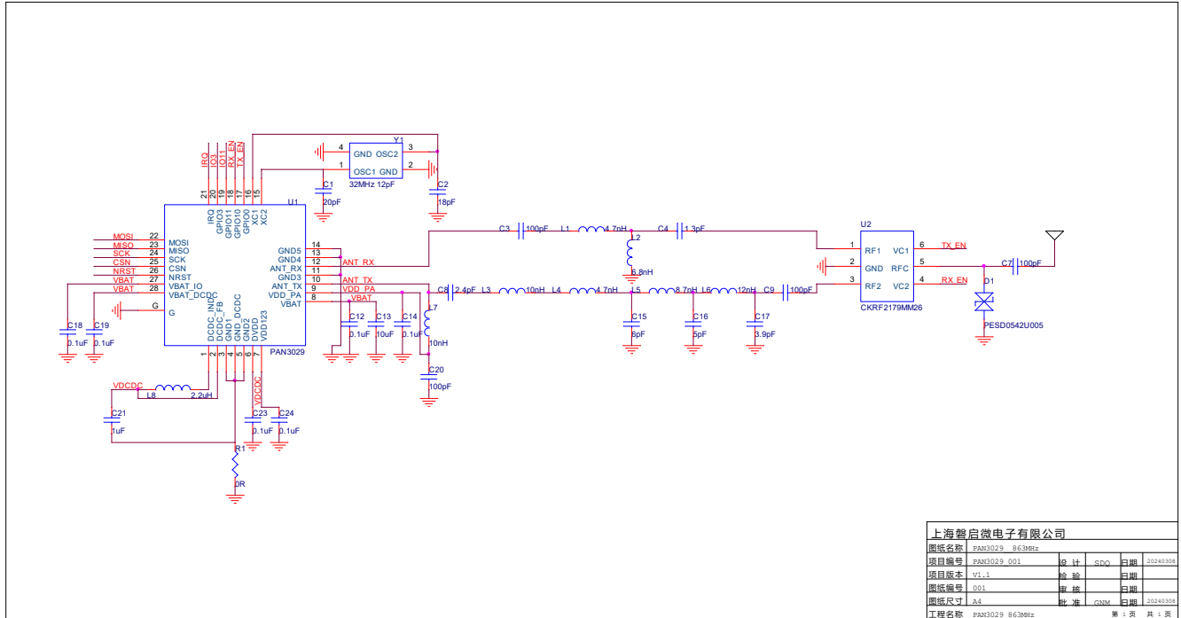
Figure 1-4 863MHz reference schematic
